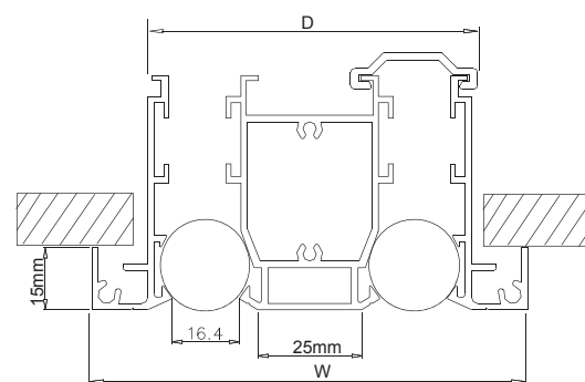
KVSLS3800 FRAME -SXS-
