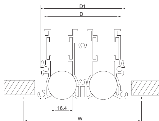
KVSLS3800 FRAME -N-
