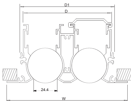
KVSLS3900 FRAME -N-
