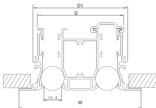
KVSLS3800 FRAME -NXN-
