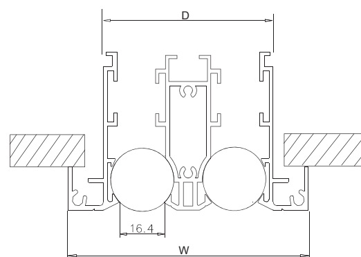
KVSLS3800 FRAME -SS-
