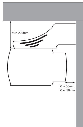
Reverse Brackets-WMB
