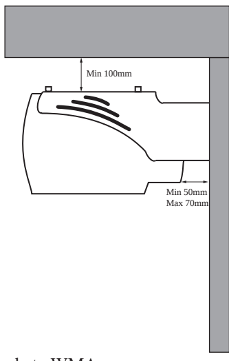
Standard Brackets-WMA
