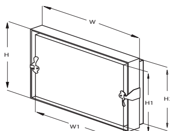
MODEL K65 (CAD) HINGELESS, FLUSH DOOR AND FLUSH MOUNT ACCESS DOOR WITH MULTIPLE CAM LOCKS FOR DOOR CLOSURE.
